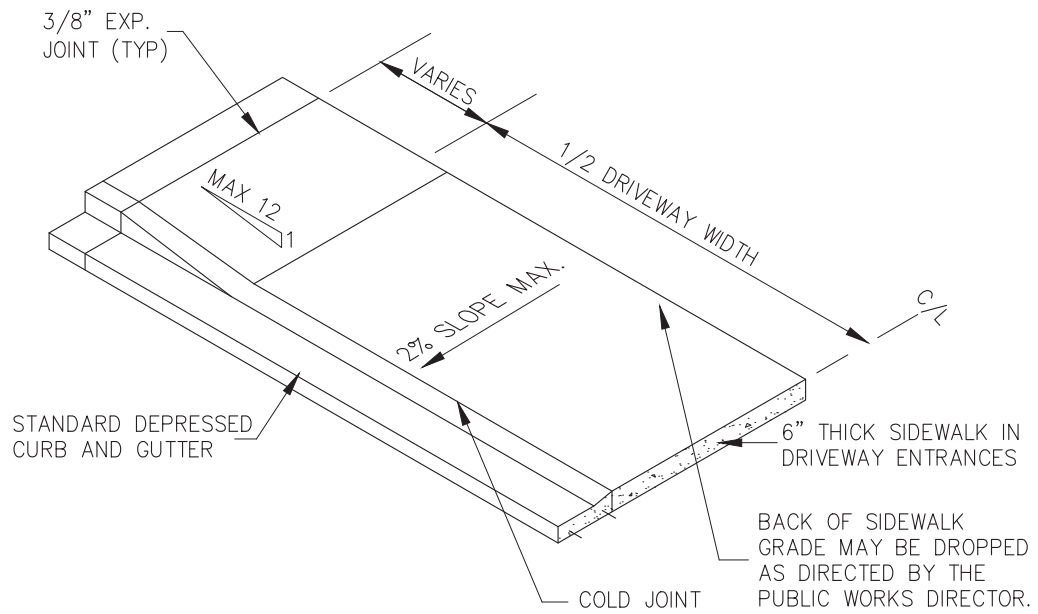
ISOMETRIC VIEW
